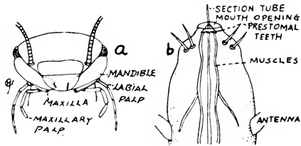
Fig. 46. a, Mouth parts of the firebrat, Thermobia domestica (Packard); b, Mouth parts of the long-nosed cattle louse, Linognathus vituli (L.).
